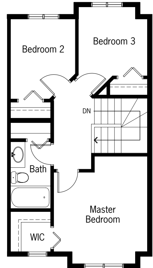
Unit A-1 Second Floor Plan 566 Sq.Ft.
