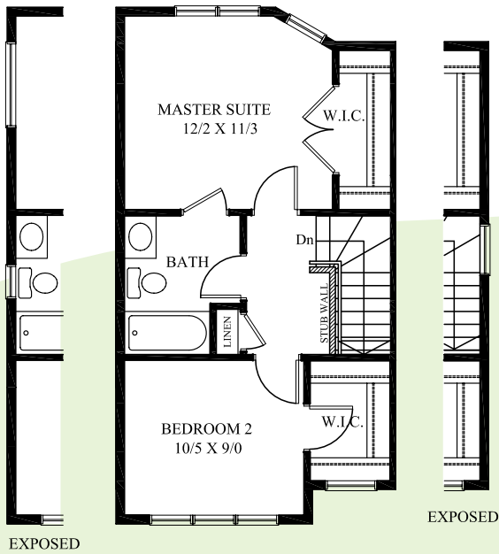
upper floor - 438 sq. ft.
