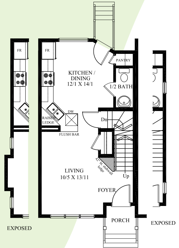
main floor - 468 sq. ft.
