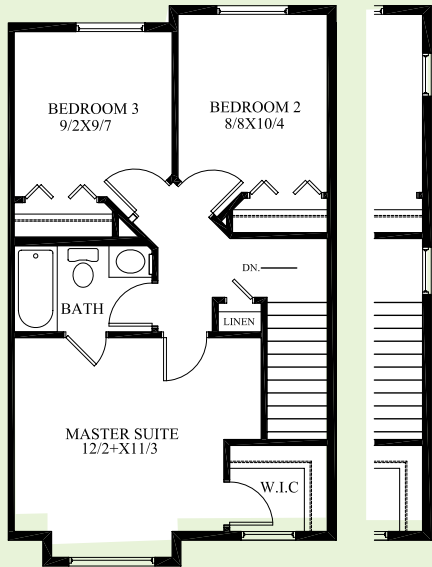
upper floor - 548 sq. ft.
